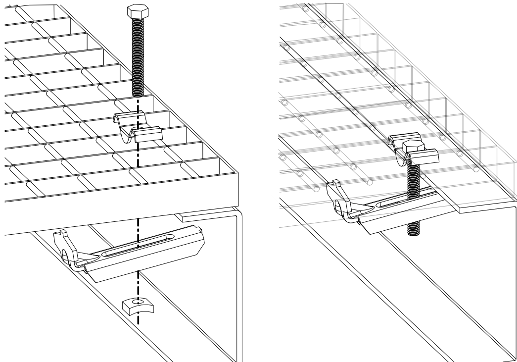
Assembly instruction - Complete fixing for grating Method shows grating Type A & U steel beam
